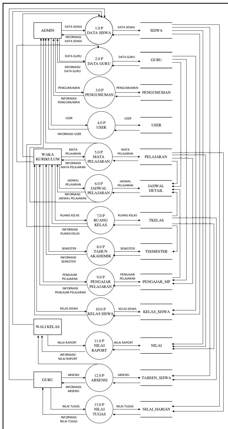
Gambar 5.10 Diagram Level 0
