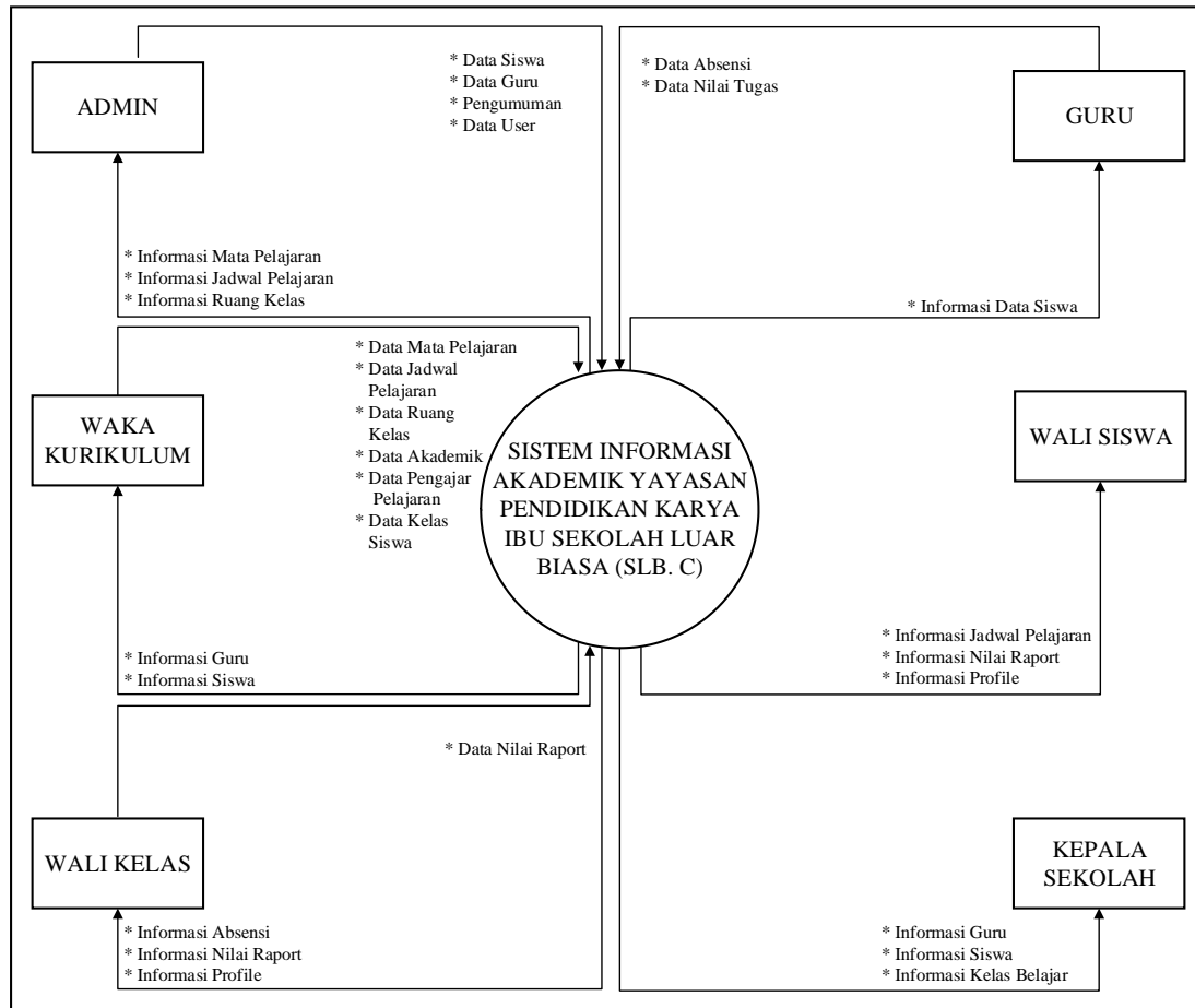
Gambar 5.9 Diagram Context
