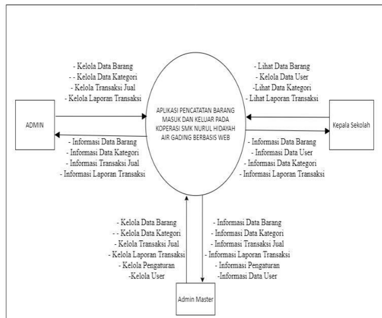
Gambar 3.5 Diagram Konteks
