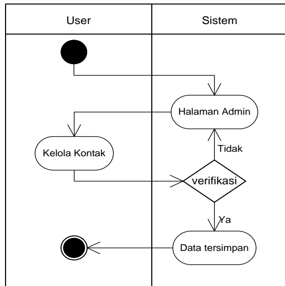
Gambar 5.12. Activity Diagram Kelola Kontak
