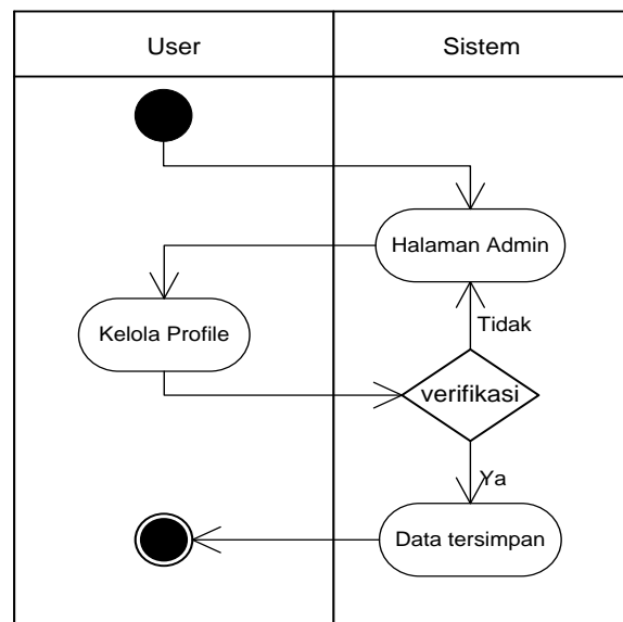
Gambar 5.6. Activity Diagram Kelola Profile
