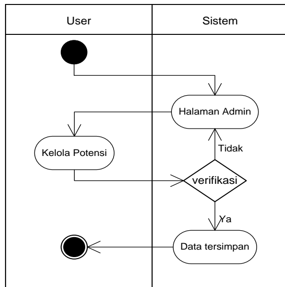
Gambar 5.10. Activity Diagram Kelola Potensi
