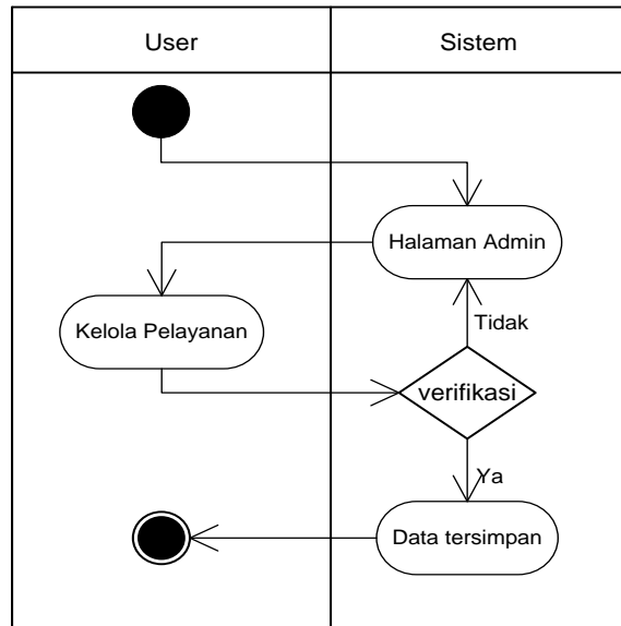
Gambar 5.11. Activity Diagram Kelola Pelayanan
