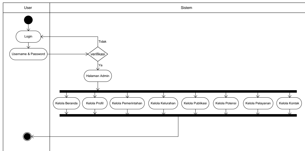
Gambar 5.4. Activity Diagram Login Admin
